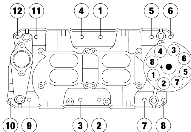
Figure 1 - 262-400 c.i.d. Small Block Chevy Torque Sequence Torque Bolts to 25 ft/lbs.
