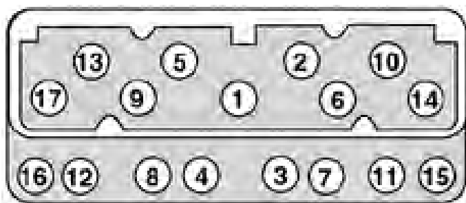
Figure 1 - SBC Cylinder Head Bolt Torque Sequence
