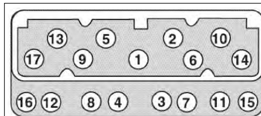
Figure 2 - Cyl. Head Bolt Torque Sequence
