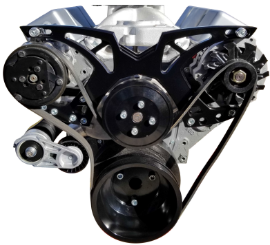
Kit21100 use a 59" 6 rib belt (Dayco 5060590)
