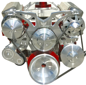
Kit 21150 with Type 2 p/s use a 62" 6 rib belt (Dayco 5060620)
