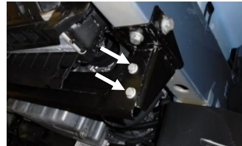
Figure 4: Mounting Location on Vehicle of Mounting Brackets
