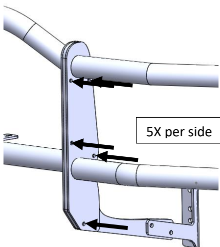
Figure 2: Assembly Hardware Locations
