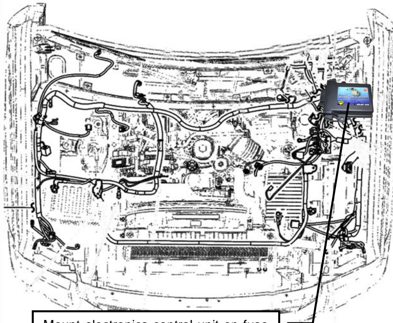
Mount electronics control unit on fuse box using Velcro.
