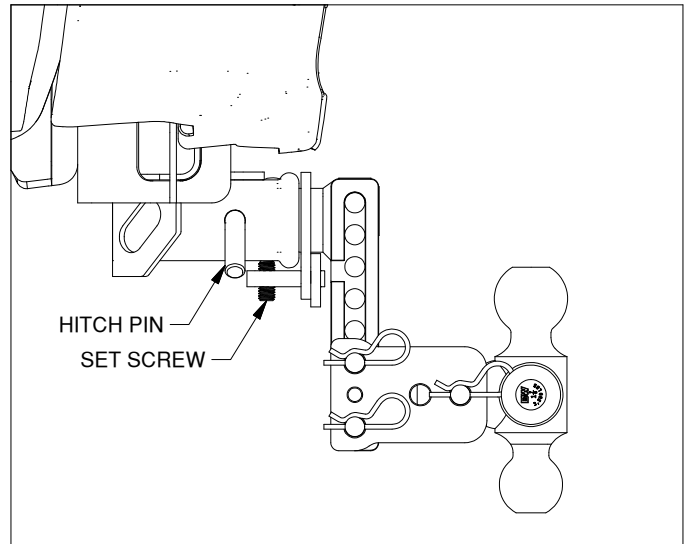
Figure B3: Towing accessory installation.
